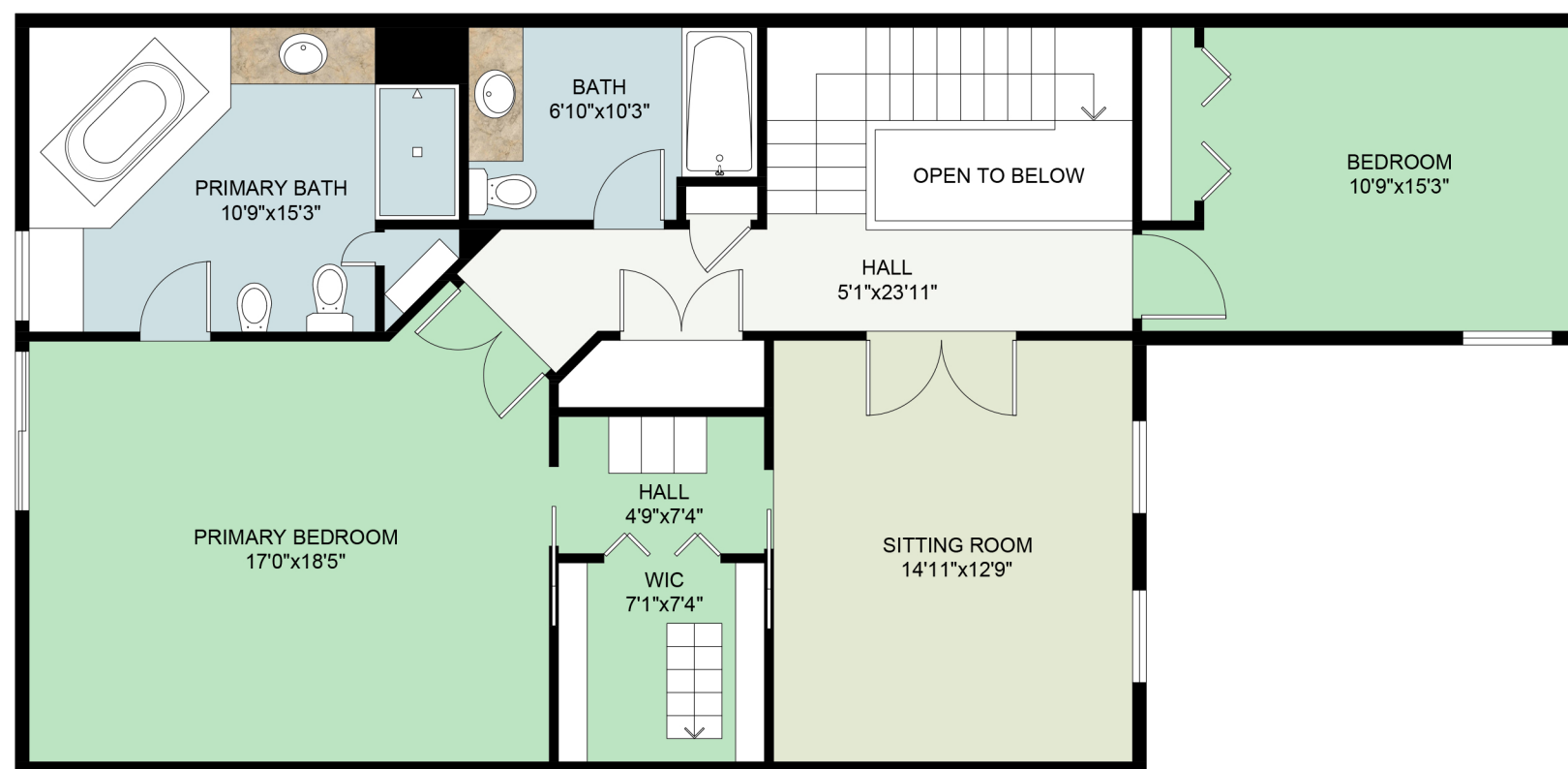
SECOND FLOOR
