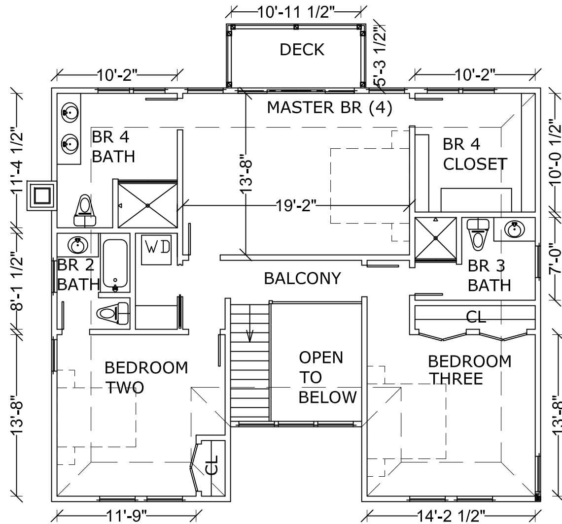
PROPOSED SECOND FLOOR PLAN 1376 SF
