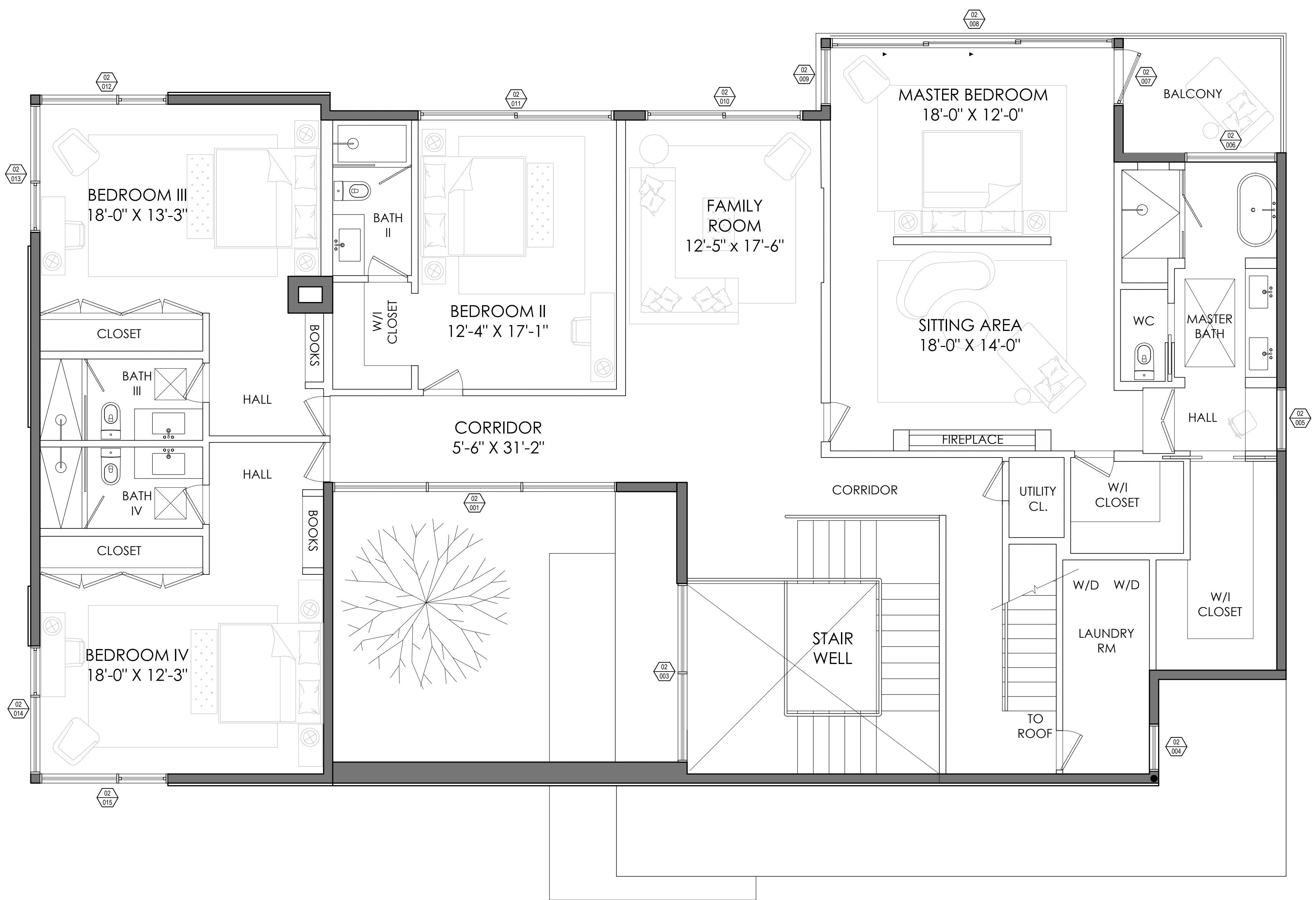
UPPER LEVEL
